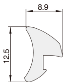
XCPB72-912 XCPB73-913 (后装面板压条)
