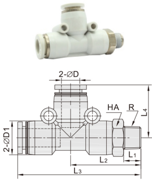
DCA11-CPD 螺纹侧三通
