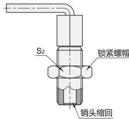
带锁紧螺帽 YZU61/YZU62
