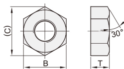
附件螺帽
