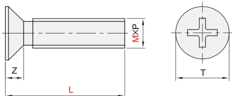
十字槽沉头螺钉 YAP01/02
