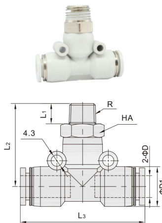
DCA04-CPB螺纹正三通
