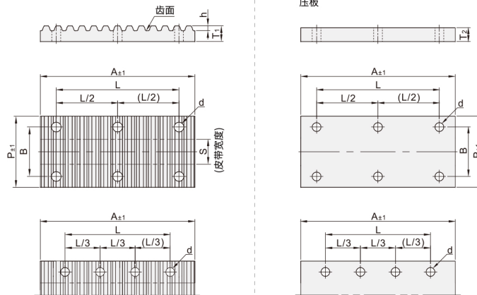
EAC11 (齿条+压板) 齿条
