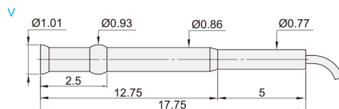
针套 ZAP01
