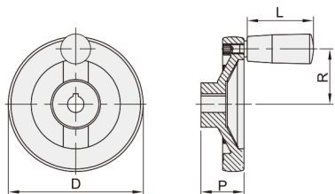
SGB11/12/13 D=60~100
