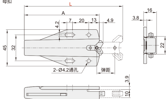
VPS82/83 母扣
