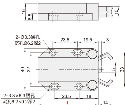
VPS81 母扣
