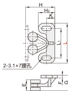
VPS21 母扣
