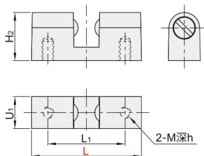
VPS16 母扣
