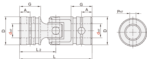
销孔型单节 CXJ01/CXJ51
