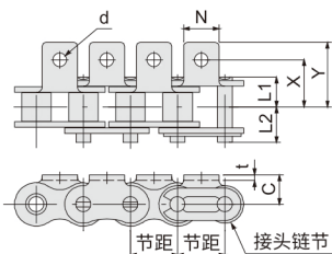
KHZ01□□B (每2节带附件)
