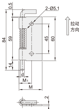
VKY21/22/23/24 规格: 17
