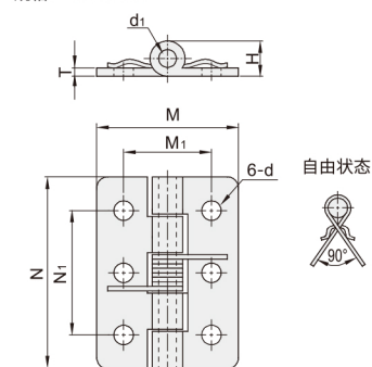
VKU22/23 规格: 6550/7550
