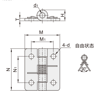
VKU22/23 规格: 4035/5035
