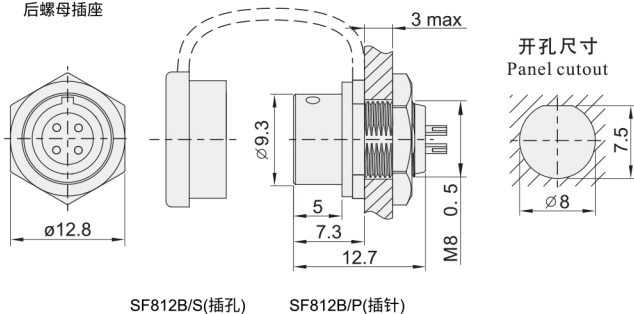
SF812B/S(插孔)
