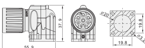
ZL 母针弯式方形法兰插座
