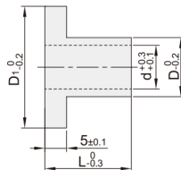
肩型轴环 SAA43
