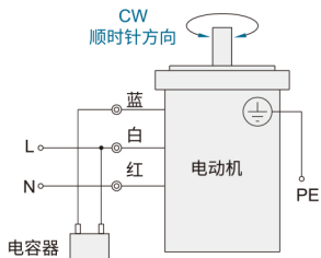
■ 接线示意图 60W, 1ph100V/110V/120V/220V/230V
