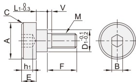
附件螺栓
