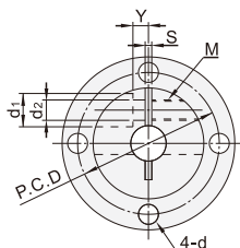
圆法兰型ZPM01/02/06
