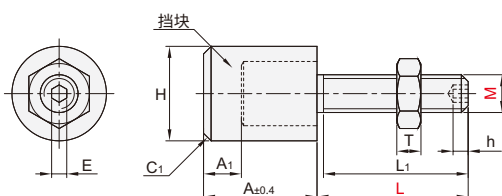
平头圆柱大挡块 YTD61/62/63/64
