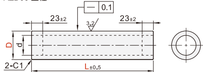
AZD06 立柱
