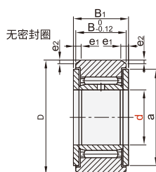
圆柱型BCN05/06
