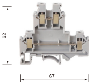
UKKB5 厚度:6.2mm
