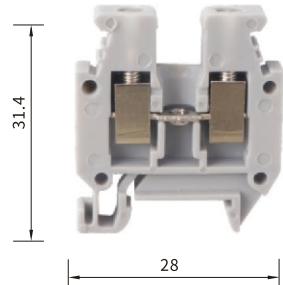
UBK3-Z 厚度:5.2mm
