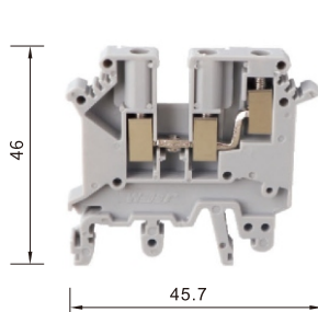
UK5-TWIN 厚度:6.2mm
