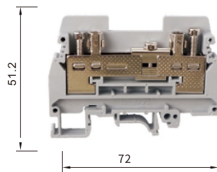
UK10-RD配保险丝R055 厚度:12.2mm
