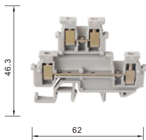
MBKKB2.5 厚度:5.2mm
