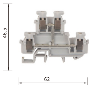
UK5-TWIN 厚度:6.2mm
