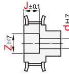
B型带轮V孔
