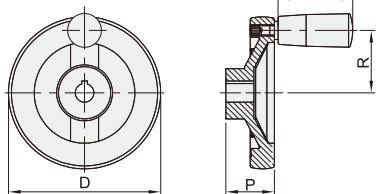
SGB11/12/13 D=60~100
