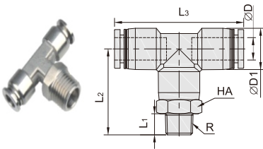
HDCC22-SSBG 螺纹正三通-G螺纹
