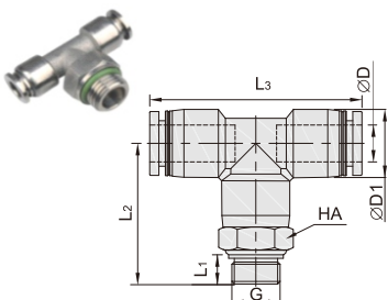
HDCC22-SSBG 螺纹正三通-G螺纹
