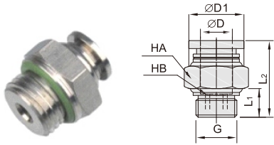
HDCC02-SSCG 螺纹直通-G螺纹
