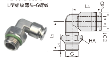
HDCC12-SSL-G L型螺纹弯头-G螺纹
