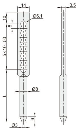
帶多孔连杆 CXAG41/42
