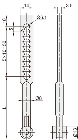
帶多孔滾輪連杆 CXAG43
