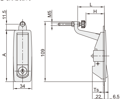
带锁芯 CXAD67/68 无锁芯 CXAD69/70
