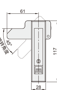
带锁芯 CXAD12 无锁芯 CXAD13
