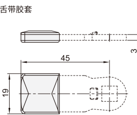
锁舌带胶套
