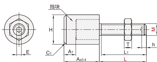
平头圆柱大挡块 YTD61/62/63/64
