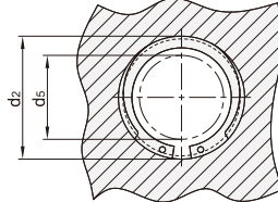
挡圈装配尺寸
