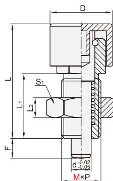
带锁紧螺帽 YZB61/YZB62
