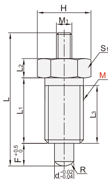
无锁紧螺帽 YZB01/YZB02
