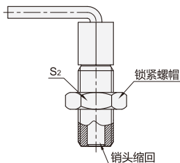
带锁紧螺帽 YZU61/YZU62
