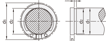
挡圈装配尺寸
