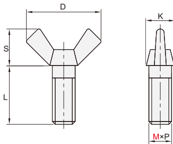
蝶型螺栓 YBB02
