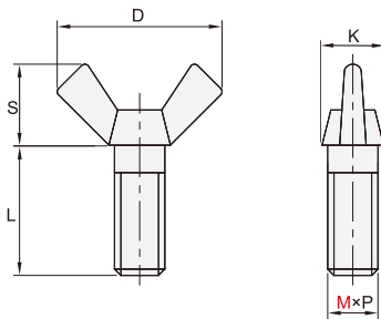
蝶型螺栓 YBB02
