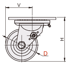
边刹 WKG02
