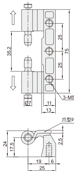
VKU91
