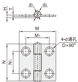
VKH13
