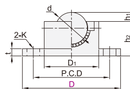
圆法兰式 LFA21/23/25/27/29
