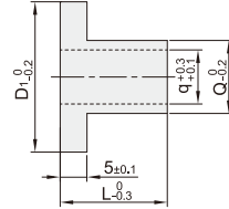
肩型轴环 SAA43
