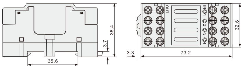
RY4N-16P-S
