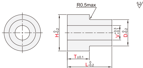
尺寸指定 EYCK21/22/23/24/25/26/37/38/39/51/61
