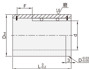
LOCTITE粘接型·直柱型 AOFF02
