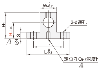
带定位孔 ZFJ21/22/26
