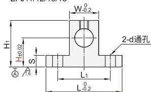
无定位孔 ZFJ01/02/06/08 ZFJ11/12/16/18
