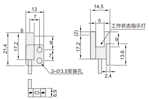
RU2-RN45 RU2-RP45
